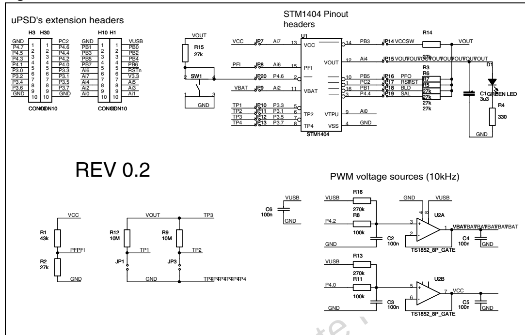
Figure 1. Schematic
